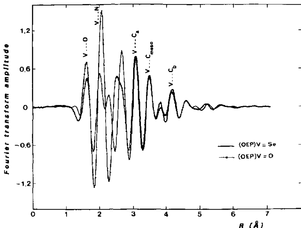
Fig. 14. Comparison of the imaginary part of the Fourier transformed spectra I_m\tilde{\chi}(R) of (OEP)V=O and (OEP)V=Se.
