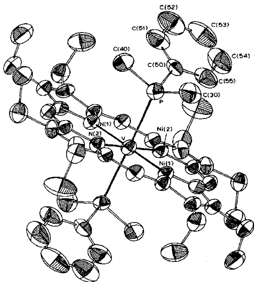
Fig. 12. ORTEP view of (OEP)V(PPhMe 2 ) 2 [58,59].
