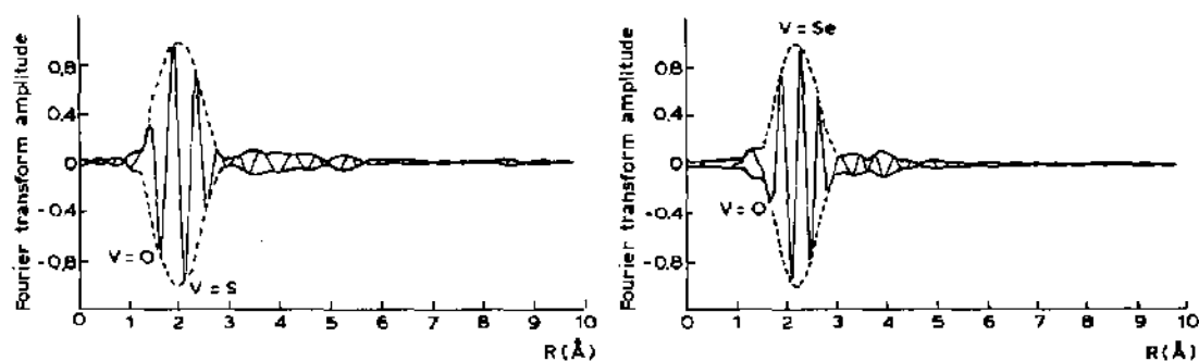
Fig. 15. Difference Fourier spectra: dotted line: |\tilde{\chi}(R)| ; full line: I_m\tilde{\chi}(R) . (a) (OEP)V=S minus (OEP)V=O. (b) (OEP)V=Se minus (OEP)V=O.
