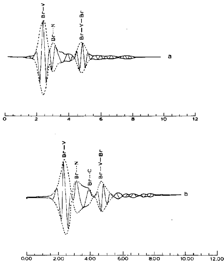
Fig. 9. EXAFS pseudo-radial distribution \hat{\chi}(R) of (\text{OEP})\text{V}(\text{Br})_2 bromine K edge. (a) Phase-shift corrections are for the \text{Br}^* \cdots \text{V} shell ( E_0 = 13468 eV). (b) Phase-shift corrections are for the \text{Br}^* \cdots \text{N} shell ( E_0 = 13474.0 eV).
